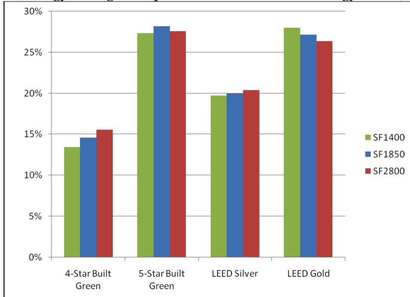
Percent Energy Savings Compared to 2006 WA State Energy Code (WSEC)
